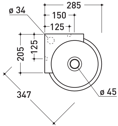
vista zenitale / zenital view
