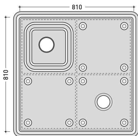
vista zenitale / zenital view art. AB4A
