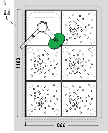
vista zenitale / zenital view art. AB6AD + 5pcs art. ABM + art. AB238
