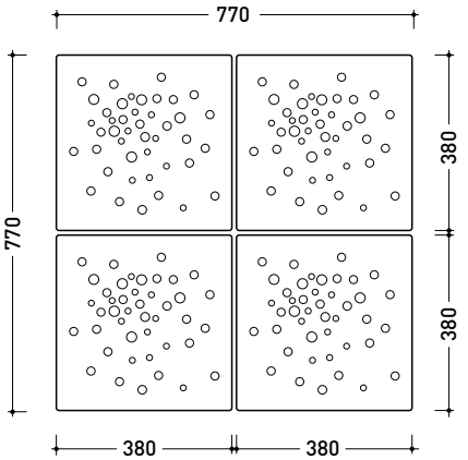
vista zenitale / zenital view 4pcs art. ABM
