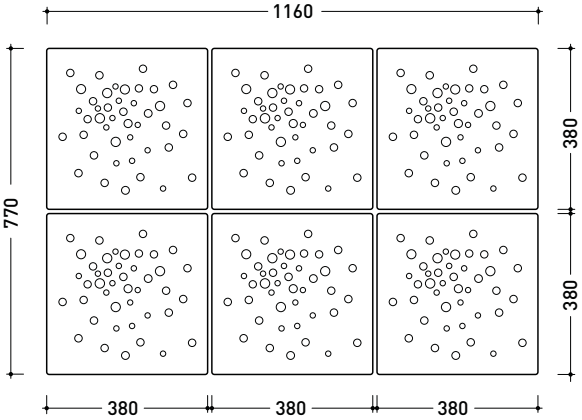
vista zenitale / zenital view 6pcs art. ABM
