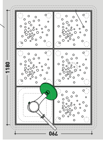
vista zenitale / zenital view art. AB6AS + 5pcs art. ABM + art. AB238
