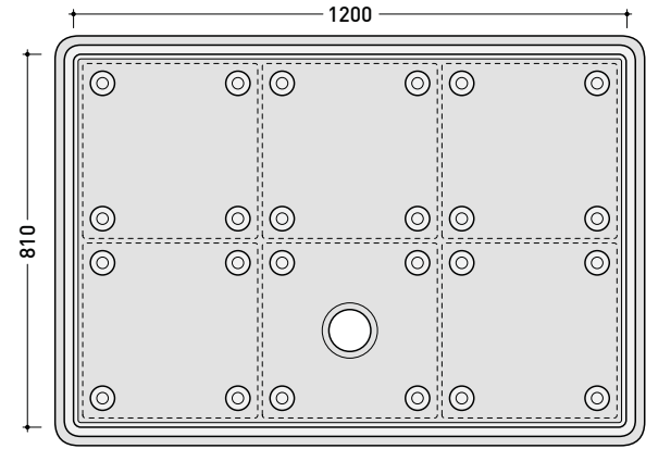
vista zenitale / zenital view art. AB6M
