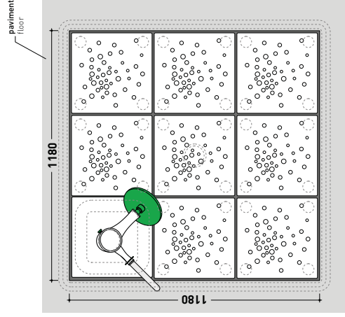
vista zenitale / zenithal view art. AB9A + 8pcs art. ABM + art. AB238
