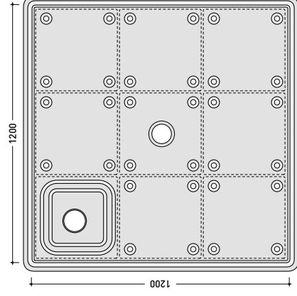
vista zenitale / zenithal view art. AB9A
