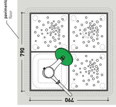
vista zenitale / zenital view art. AB4A + 4pcs art. ABM + art. AB238
