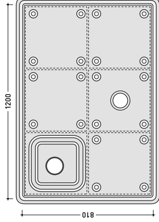
vista zenitale / zenital view art. AB9A
