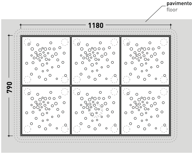
vista zenitale / zenital view art. AB6M + 6pcs art. ABM
