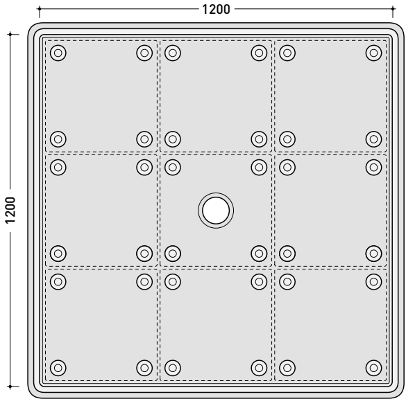
vista zenitale / zenital view art. AB9M
