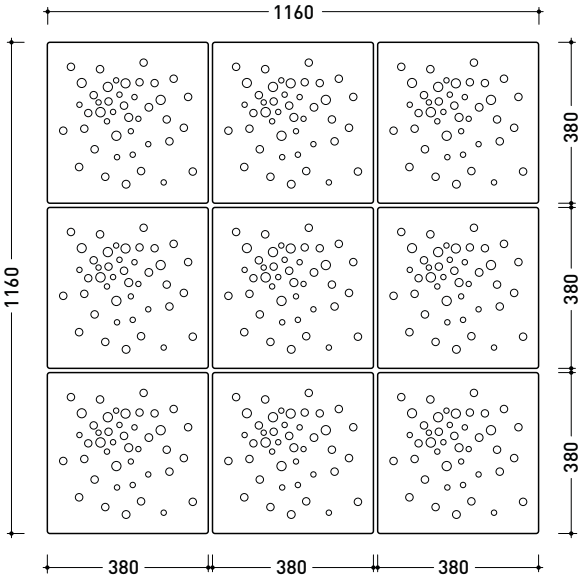
vista zenitale / zenital view 9pcs art. ABM
