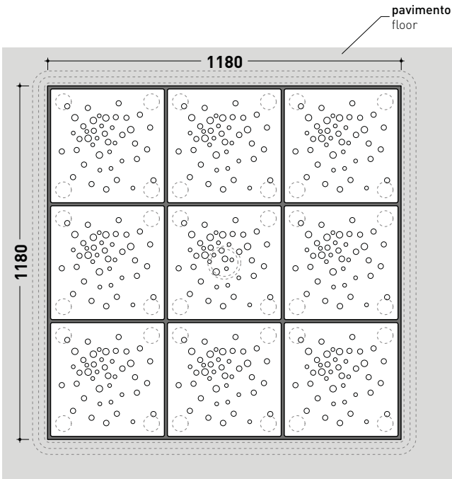
vista zenitale / zenital view
