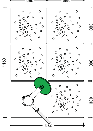
vista zenitale / zenital view 8pcs art. ABM + art. AB238
