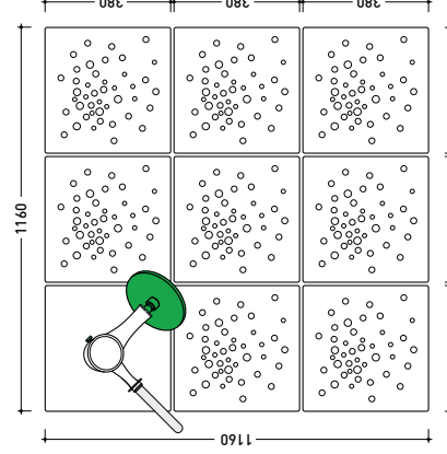
vista zenitale / zenithal view 8pcs art. ABM + art. AB238
