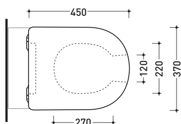
art. AP114S - AP117RS vista zenitale / zenital view
