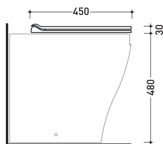
art. AP114S - AP117RS vista laterale / lateral view
