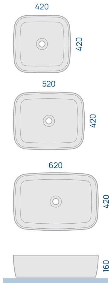
art. PY42A / PY52A / PY62A Lavabo da appoggio Countertop basin
