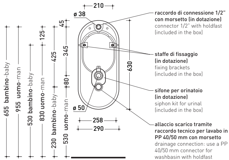
vista retro/ back view
