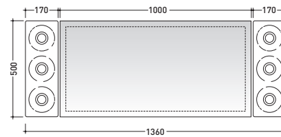
vista frontale / frontal view 2pcs art. MKLP + art. MKS501
