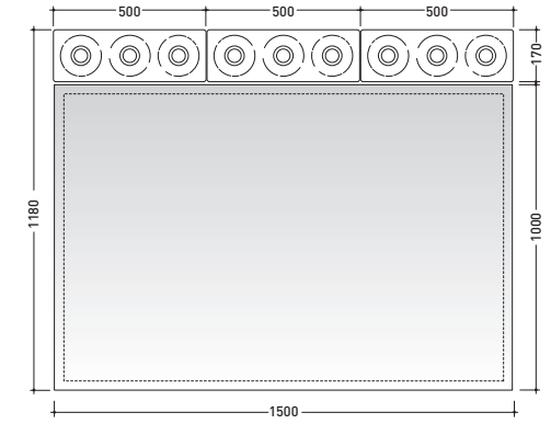
vista frontale / frontal view 3pcs art. MKLP + art. MKS100
