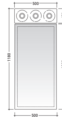
vista frontale / frontal view 3pcs art. MKLP + art. MKS50
