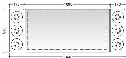
vista frontale / frontal view 2pcs art. MKLP + art. MKS501
