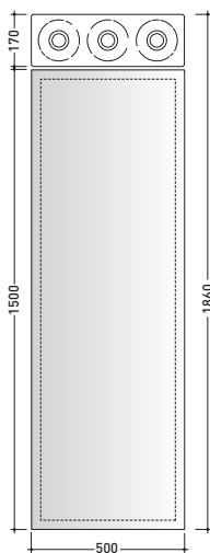
vista frontale / frontal view 1pcs art. MKLP + art. MKS501
