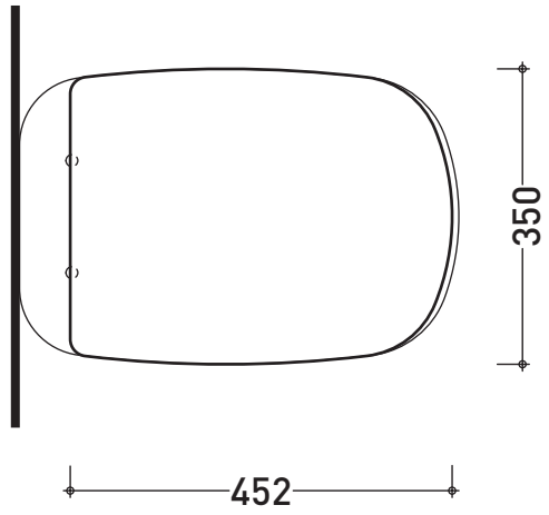
art. MN117 vista zenitale / zenital view
