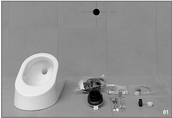
01 Allestimento / Arrangement
