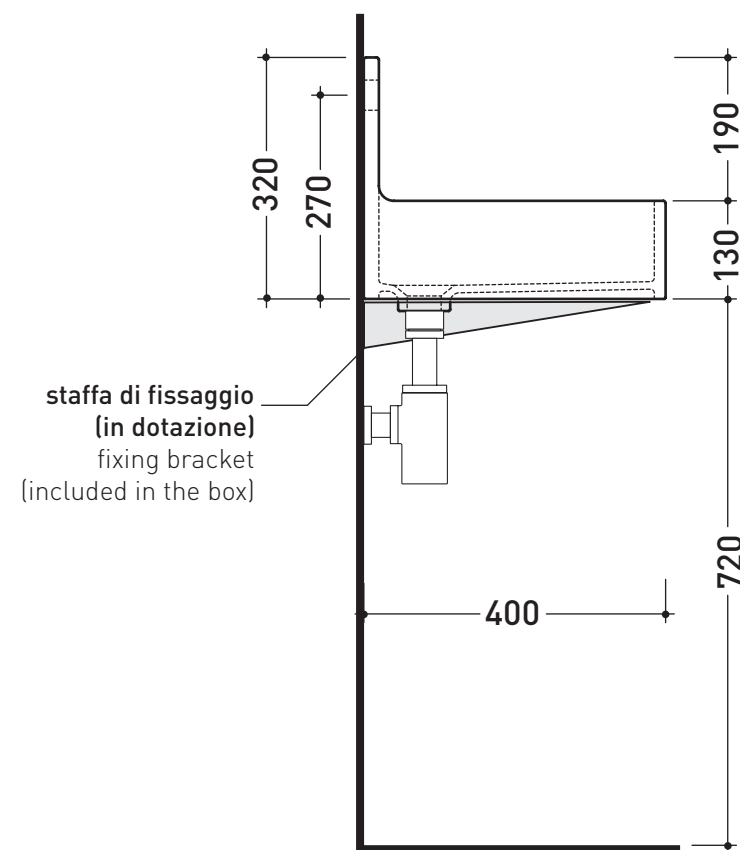
vista laterale / lateral view
