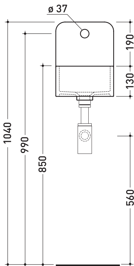
vista frontale / frontal view
