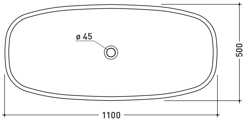
vista zenitale / zenital view
