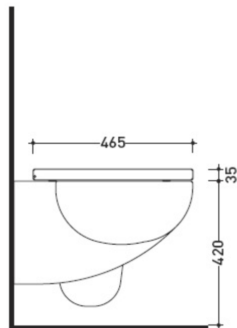
art. SR118 vista laterale / lateral view
