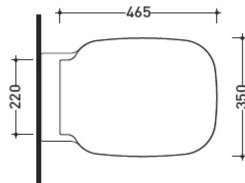
art. SR118 vista zenitale / zenital view
