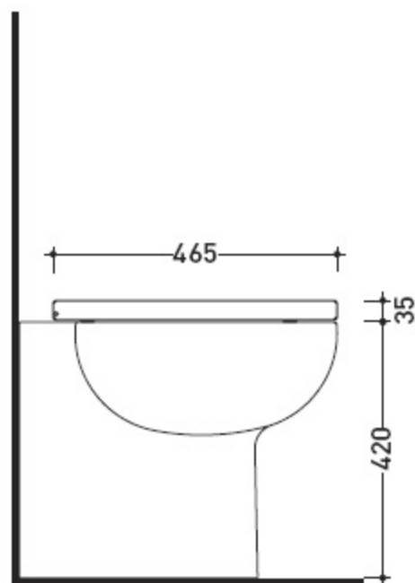
art. SR117 vista laterale / lateral view
