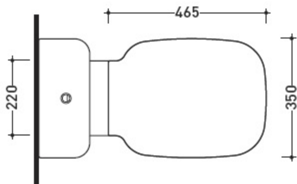
art. SR116 vista zenitale / zenital view
