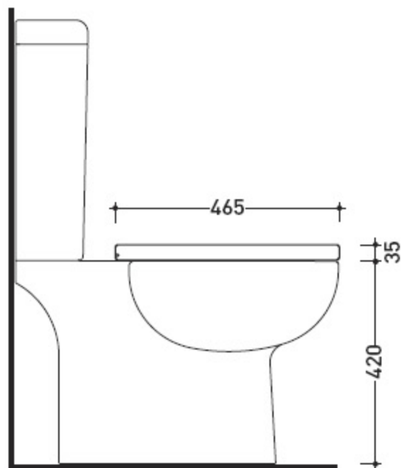
art. SR116 vista laterale / lateral view
