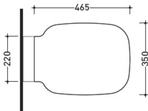
art. SR117 vista zenitale / zenital view
