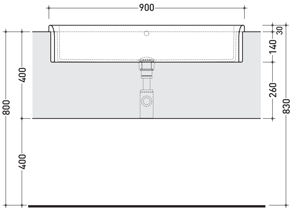
vista frontale / frontal view
